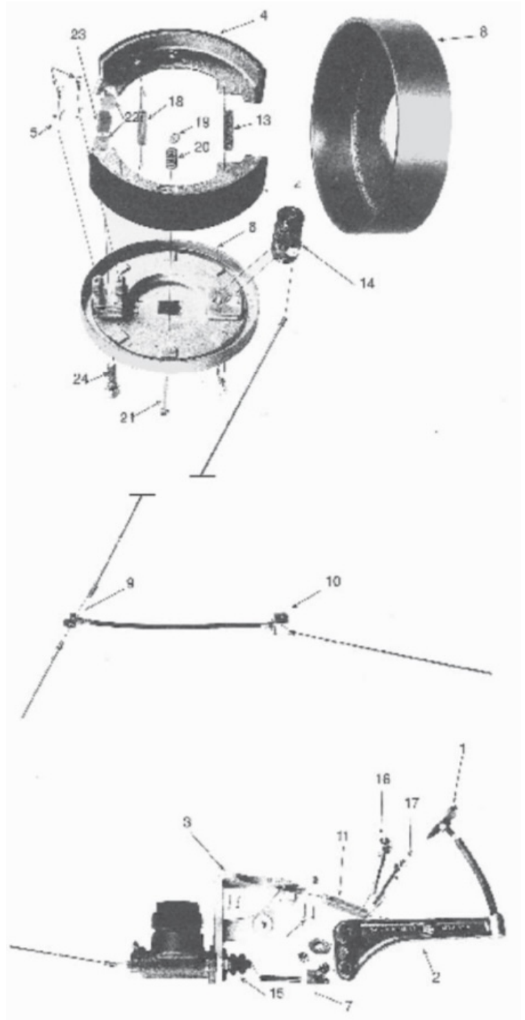
Hydraulic Brake
